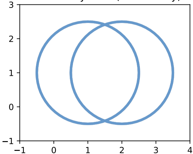
a.boundary.union(b.boundary)
