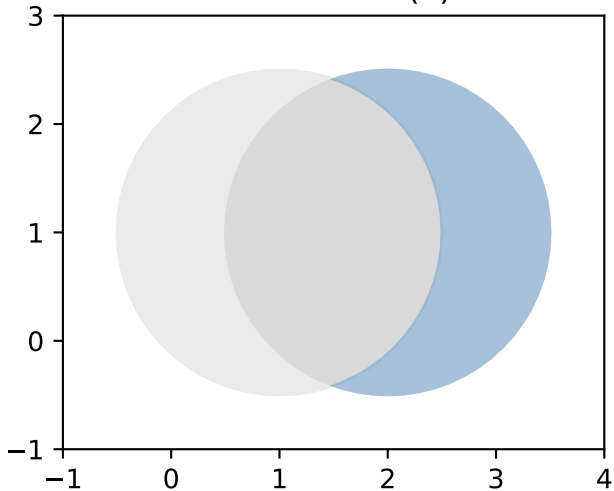
b.difference(a)
