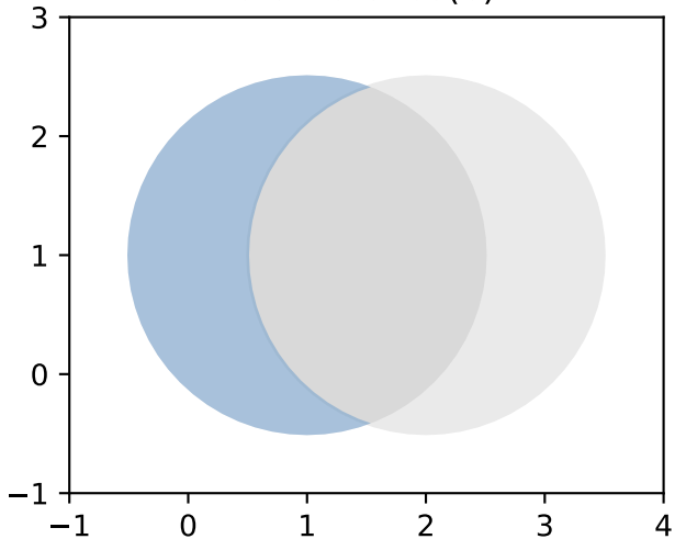
a.difference(b)
