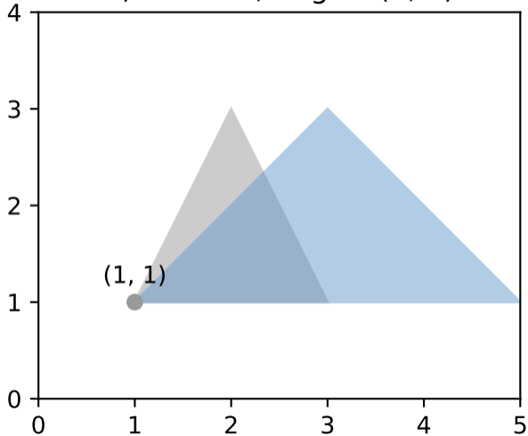
b) x\text{fact}=2 , \text{origin}=(1, 1)
