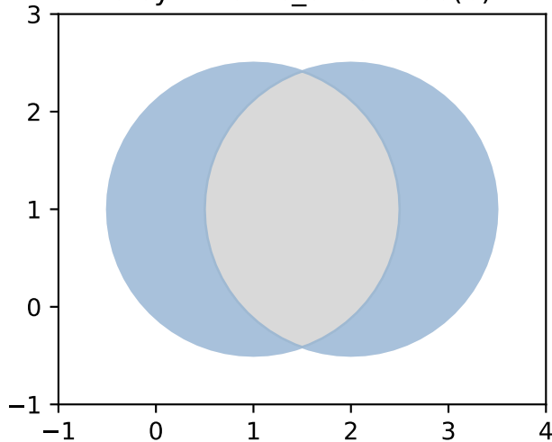
a.symmetric_difference(b)
