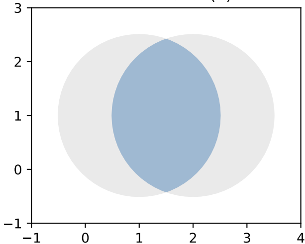
a.intersection(b)
