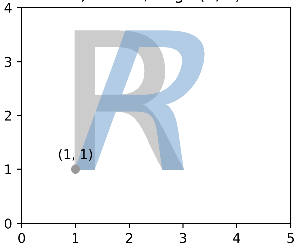
a) x_s=20 , origin(1, 1)
