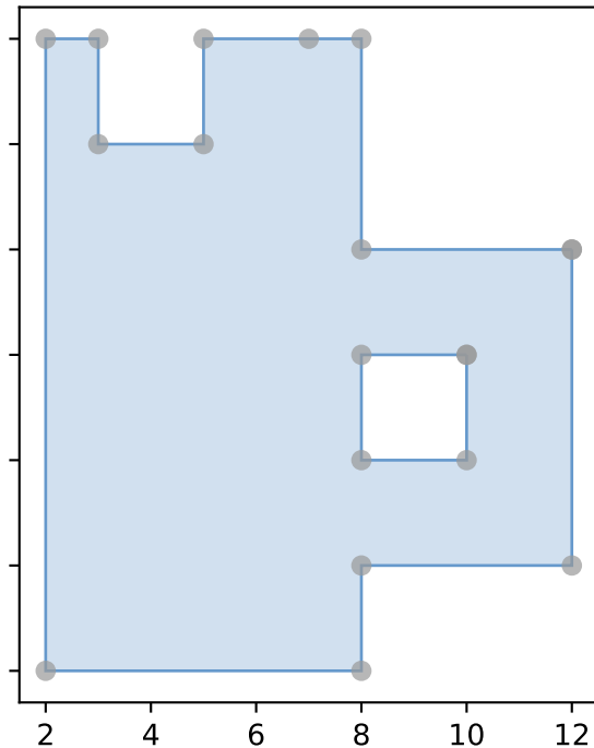
make_valid - structure
